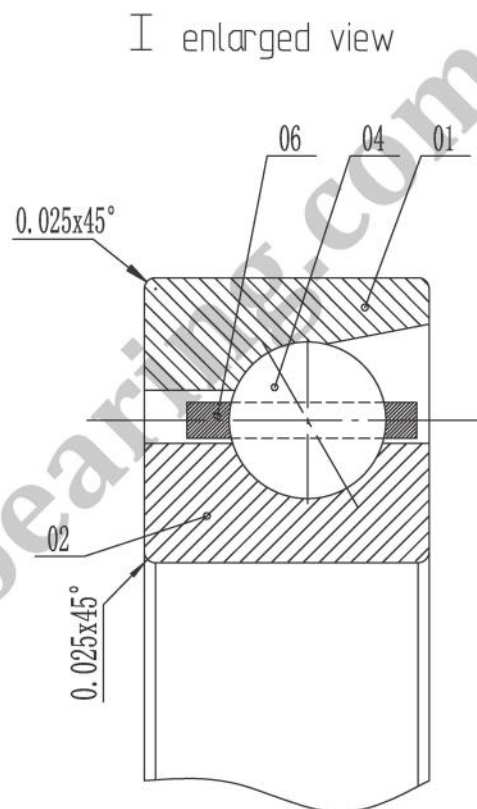
KAYDON THIN SECTION BEARING
